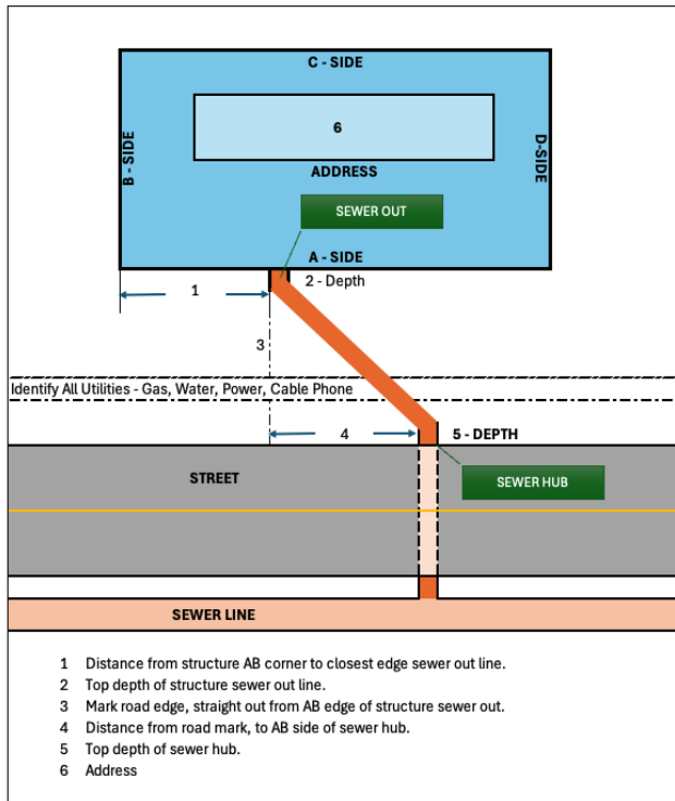
STRUCTURE SEWER CONNECTION DRAWING
